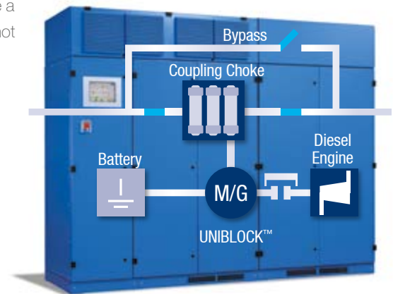
UBTD+ with external battery ride-through.
